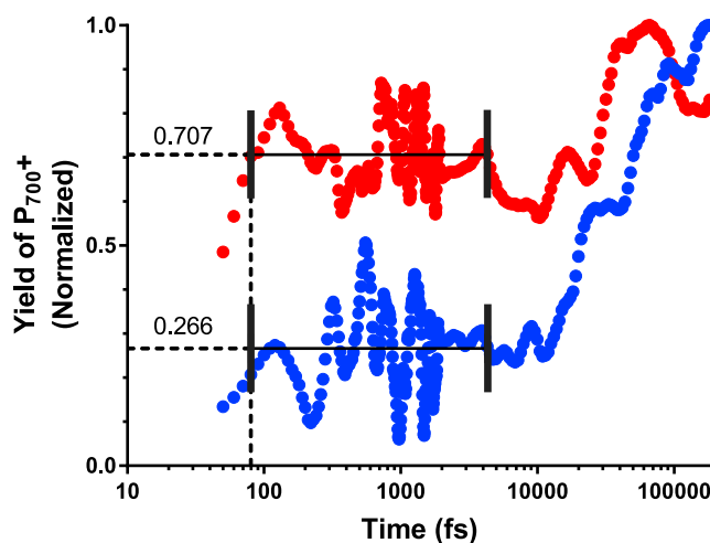
FIGURE 7 The contribution \chi(t) of the ionic state P_{700}^+ to the transient spectra \Delta A(\lambda, t) of DM-PSI (blue) and SMA-PSI (red) complexes from T. elongatus excited by a long-wave pulse of 740 nm (see Fig. S3 for details). The solid lines indicate the average between the vertical bars. Dotted lines are extrapolations back to x and y axes. The numerical values correspond to the ratio of P_{700}^+ produced in the timescale of 0.1–5 ps. To see this figure in color, go online.
