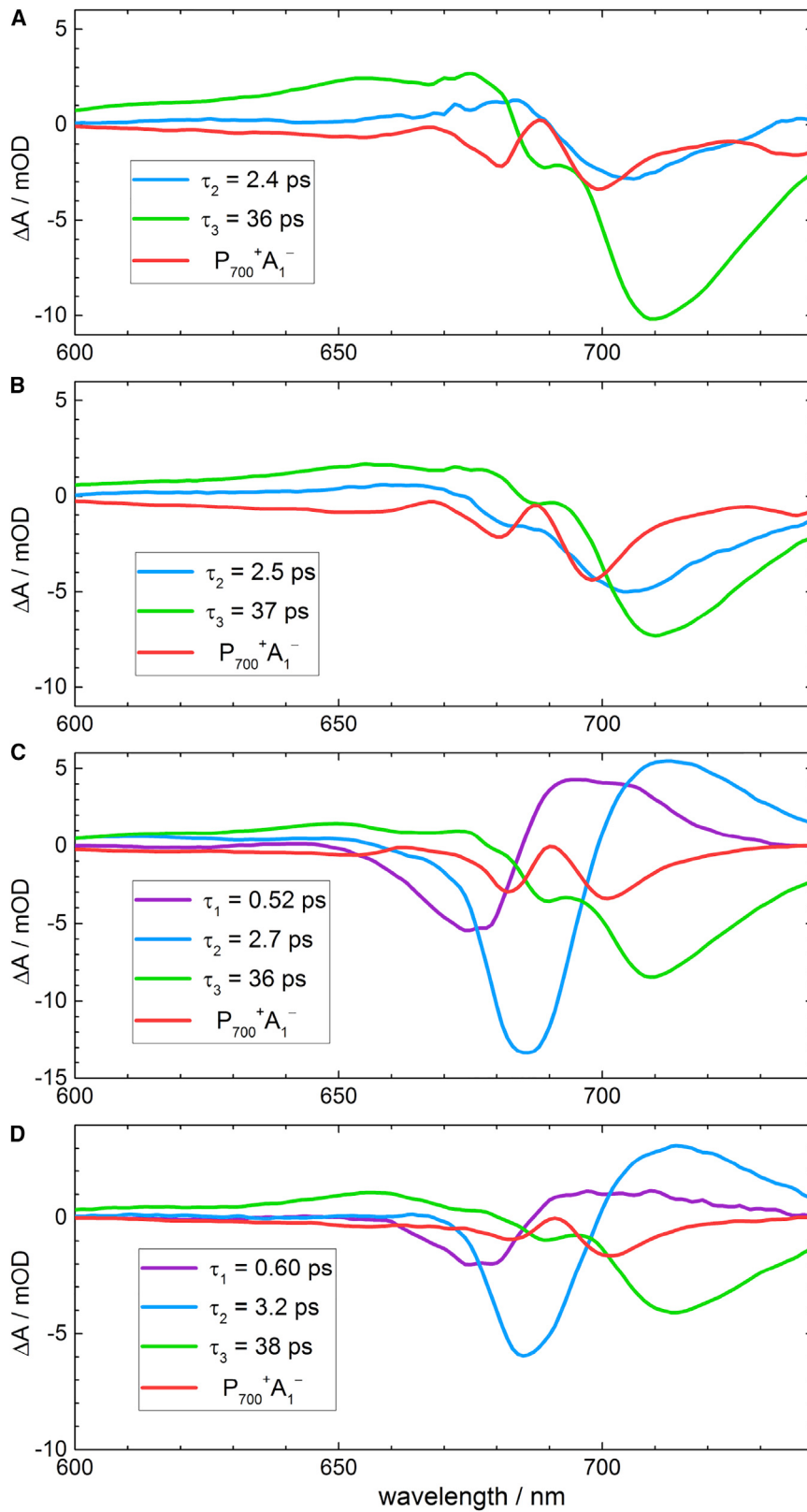
FIGURE 5 Exponential deconvolution of the transient spectral dynamics in PSI preparations from T. elongatus excited by pulses at 740 nm (A and B) and 670 nm (C and D). DM-PSI (A and C) or SMA-PSI (B and D) complexes are shown. To see this figure in color, go online.
